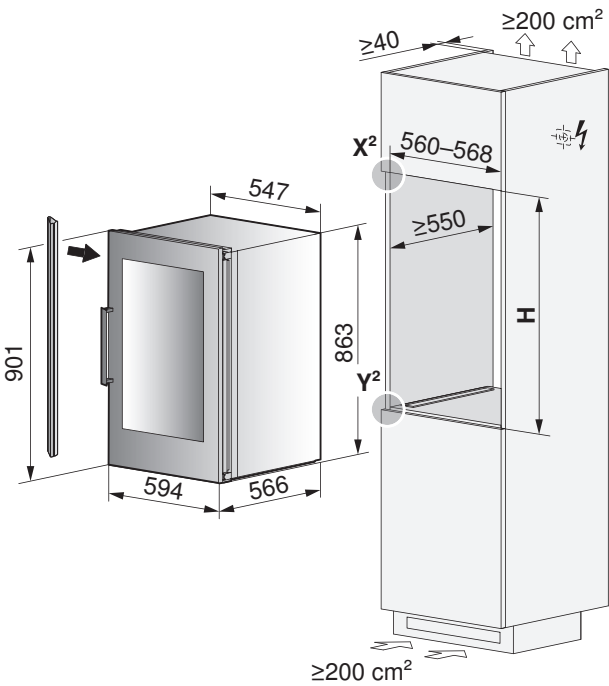
Winecooler 90 SL 60 (51094)
