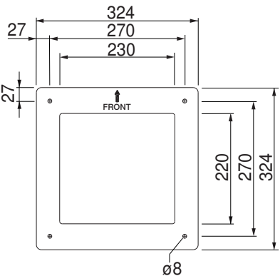
Drilling plan (view X)
