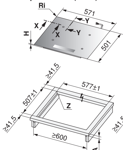
CookTop V2000 I604 (31141), CookTop V4000 I604 (31115)
